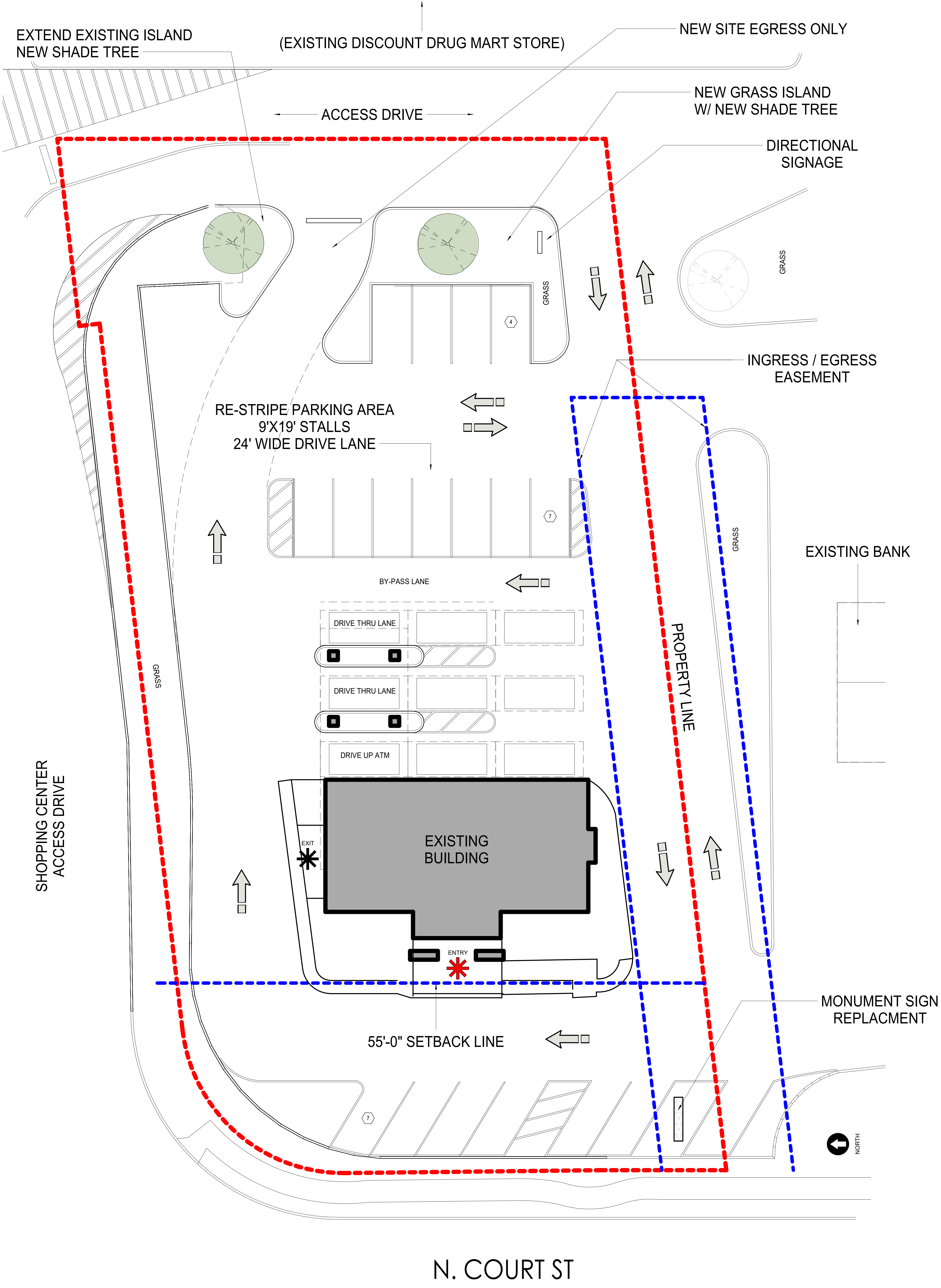
1 SITE PLAN - NEW SCALE: 1" = 10'-0"
