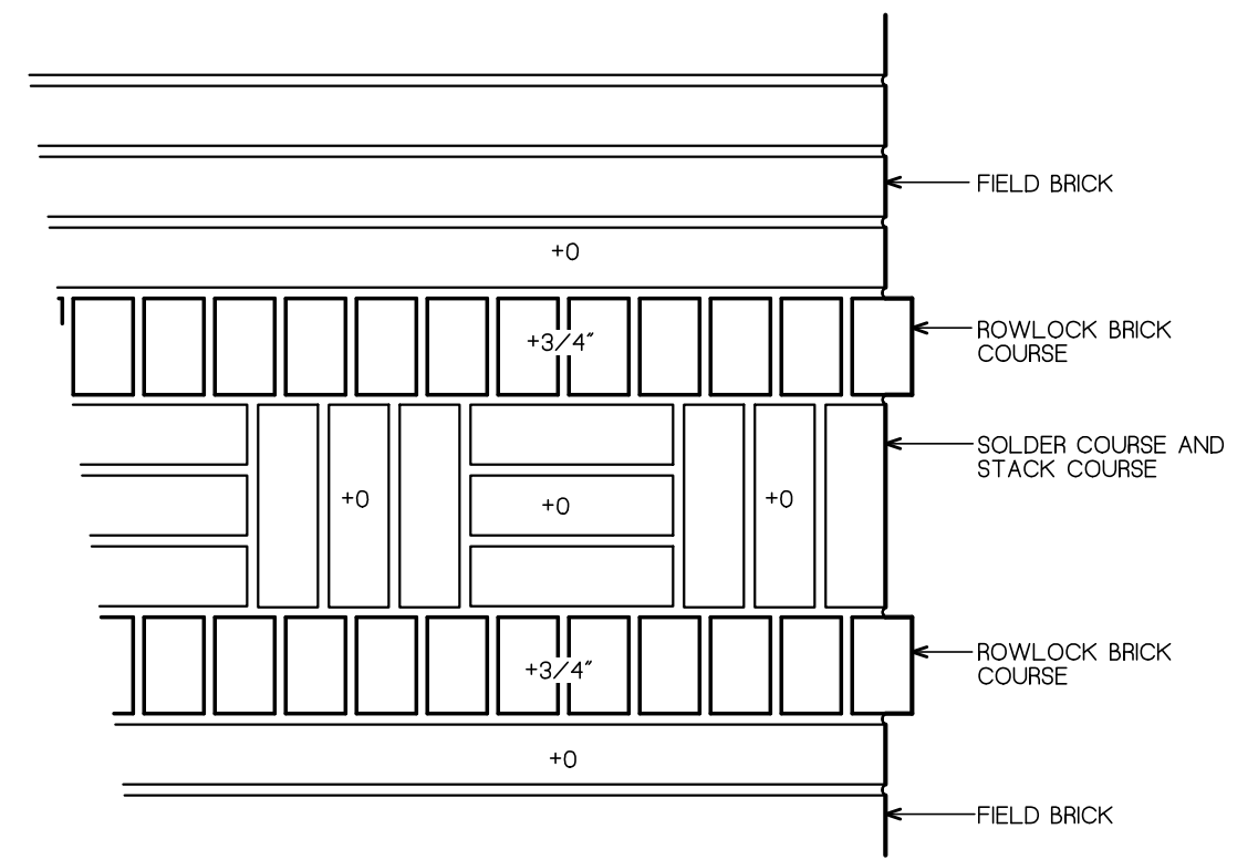
BRICK BASKETWEAVE SCALE: 1-1/2" = 1'-0"
