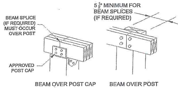
FIGURE 507.5.1(1) DECK BEAM TO DECK POST
